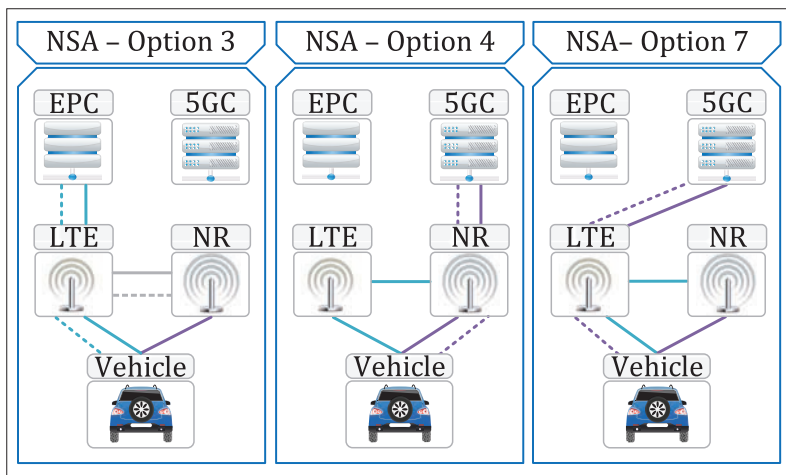
FIGURE 3. NSA deployment options for 5G NR.
