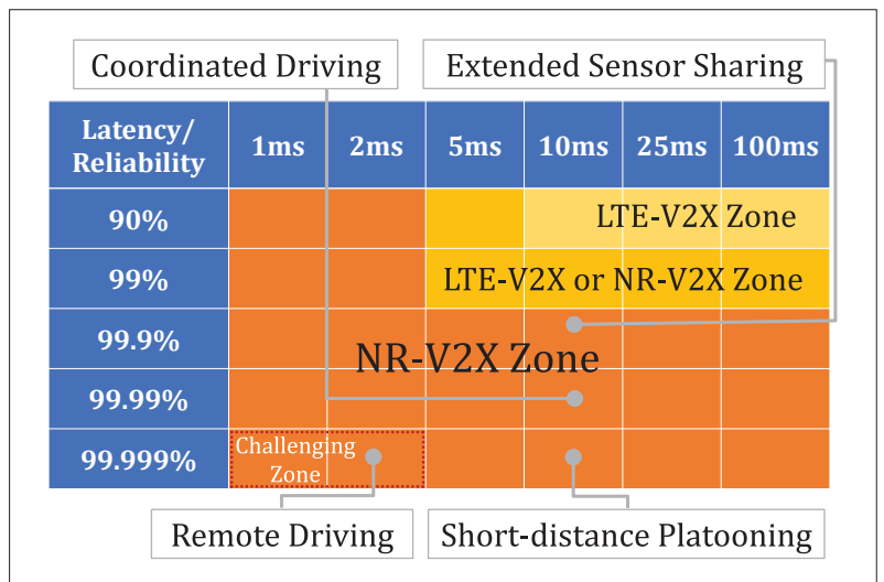
FIGURE 4. End-to-end latency and reliability requirements for advanced NR-V2X use cases.
